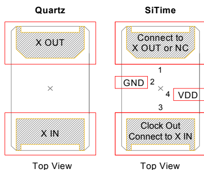
Figure 2. SiT1533 Footprint Compatibility with Quartz XTAL Footprint [6]
