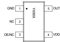
Figure 1. Pin Assignments
