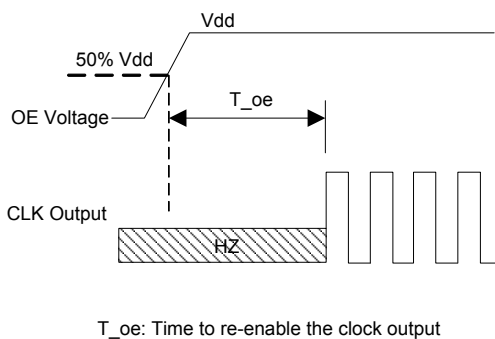
Figure 6. OE Enable Timing (OE Mode Only)
