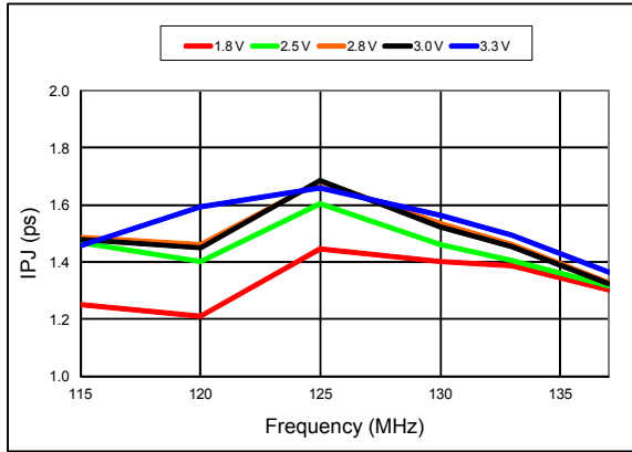
Figure 13. RMS Integrated Phase Jitter Random (12k to 20 MHz) vs Frequency [11]
