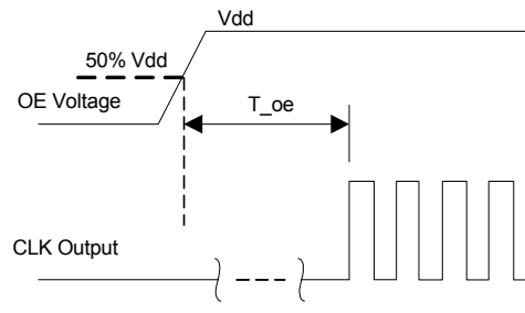
Figure 5. OE Enable Timing (OE Mode Only)
