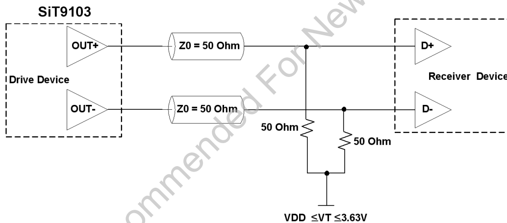
Figure 8. CML Single Load Termination
